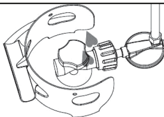
Regulator/Cylinder Connection
